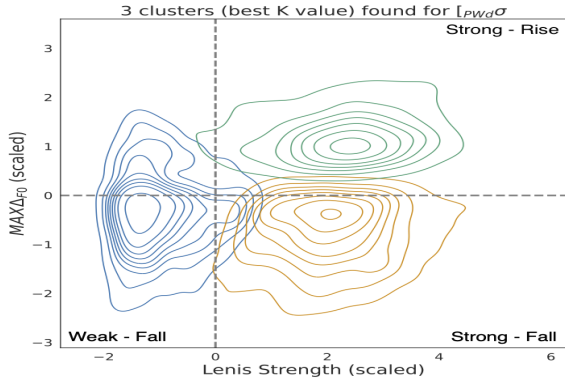
Figure 2: The three found sub-categories of [PWd\sigma , from the K-means clustering analysis
