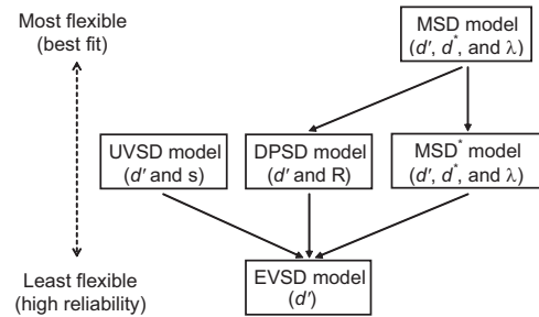
Figure 2. Nested hierarchy for the signal-detection models. Unidirectional, solid-line arrows indicate subset relations between models. The bidirectional, dotted-line arrow on the left-hand side represents the degree of flexibility and reliability. UVSD = unequal-variance signal detection; DPSD = dual-process signal detection; MSD = mixture signal detection; MSD* = subset of the MSD model where d^* = 0 ; EVSD = equal-variance signal detection; d' = sensitivity; d^* = sensitivity for partially or not attended items; \lambda = mixing probability; s = slope of the receiver-operating characteristic; R = recollection.
