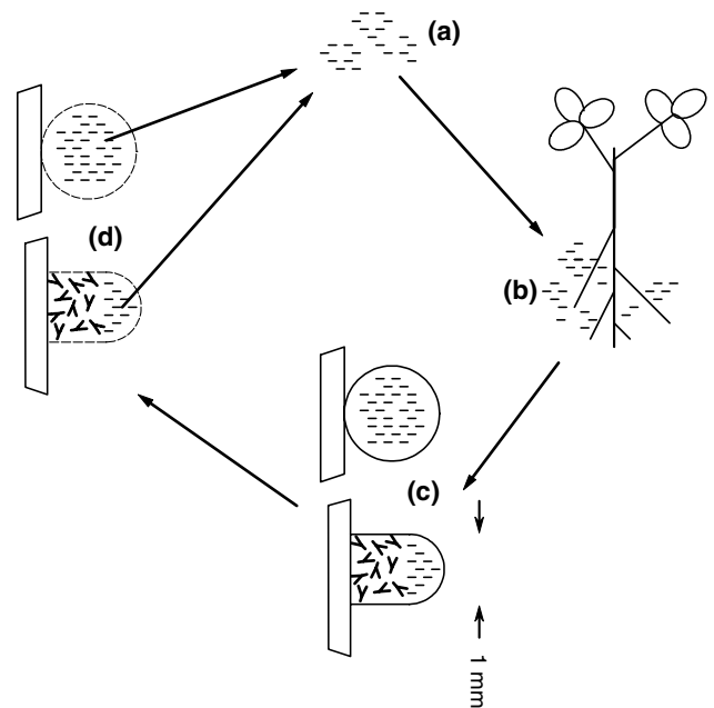
Fig. 1. Life cycle of symbiotic rhizobia: (a) rhizobia in the soil; (b) rhizobia competing for opportunities to nodulate a legume root; (c) determinate and indeterminate nodules, showing increased size and altered shape of bacteroids in indeterminate nodules; (d) senescing nodules with release of rhizobia (bacteroids from determinate nodules and undifferentiated cells from indeterminate nodules). Rhizobium numbers in nodules are much greater than shown, whereas their size is much less.
